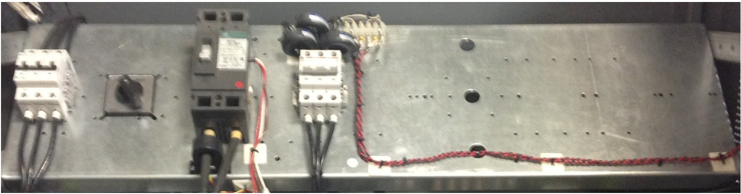
Figure 7a Main Breaker Shelf
