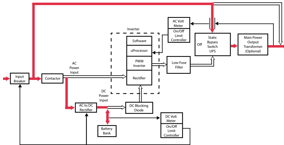
Figure 2 Single Line Drawing - Static Bypass Operation
